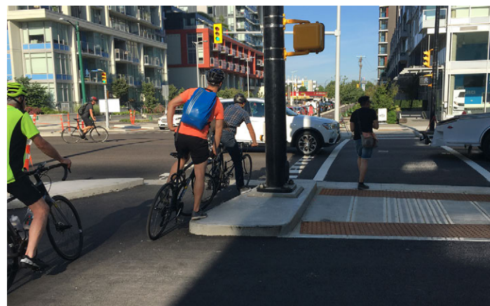
Image 6.8. Vancouver protected intersection with raised island and traffic infrastructure
