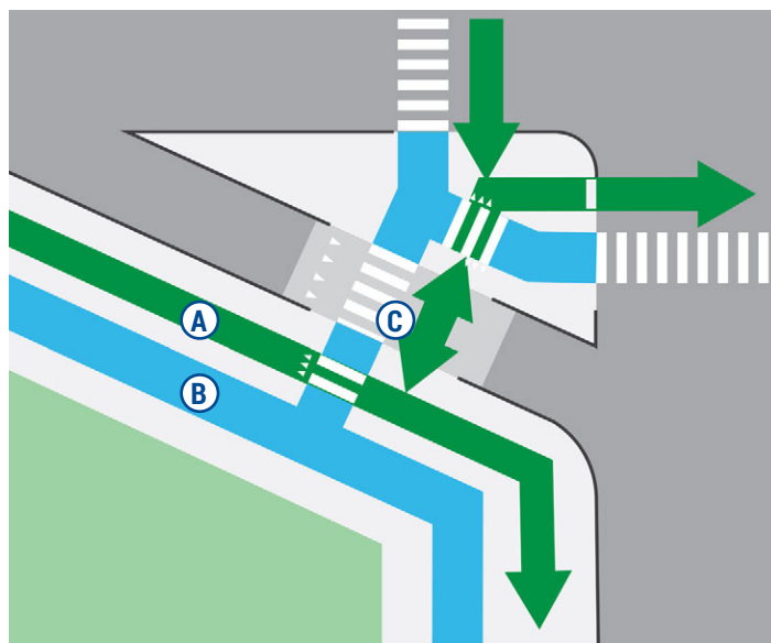
Figure 4.6. Smart channel protected corner
