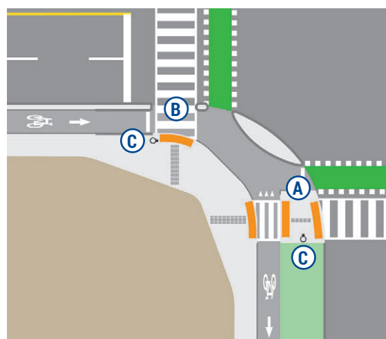
Figure 5.2. Hybrid protected intersection showing pedestrian crossings with and without a refuge
