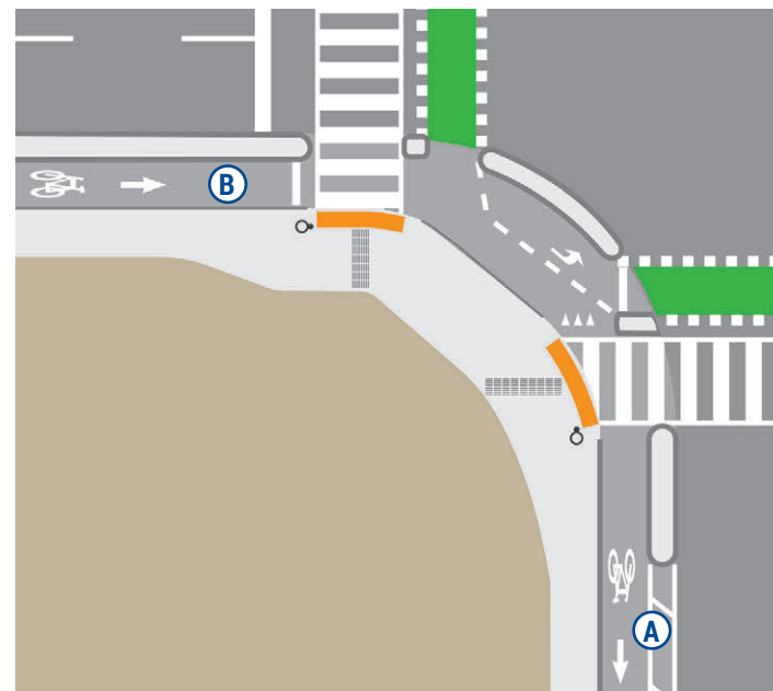
Figure 5.11. One-stage protected corner showing transition to buffered bike lane
