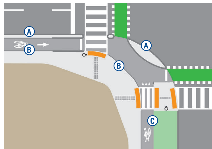
Figure 6.4. Hybrid protected corner showing relative curb heights
